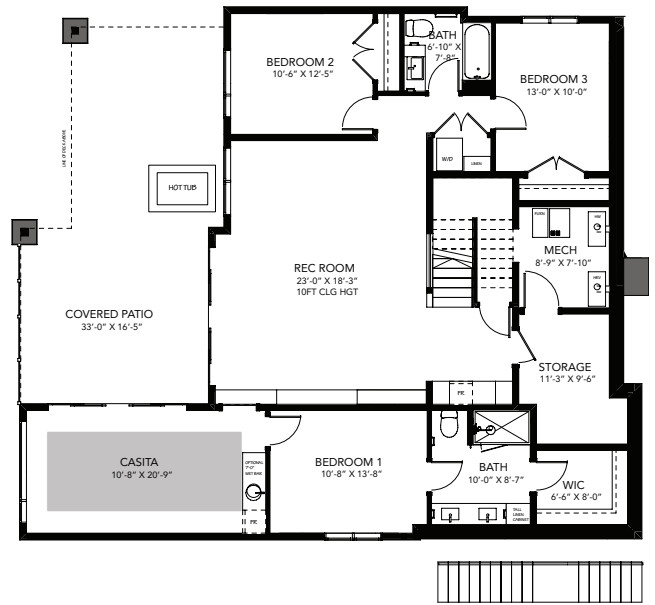
BASEMENT AREA 1,838 SQFT
