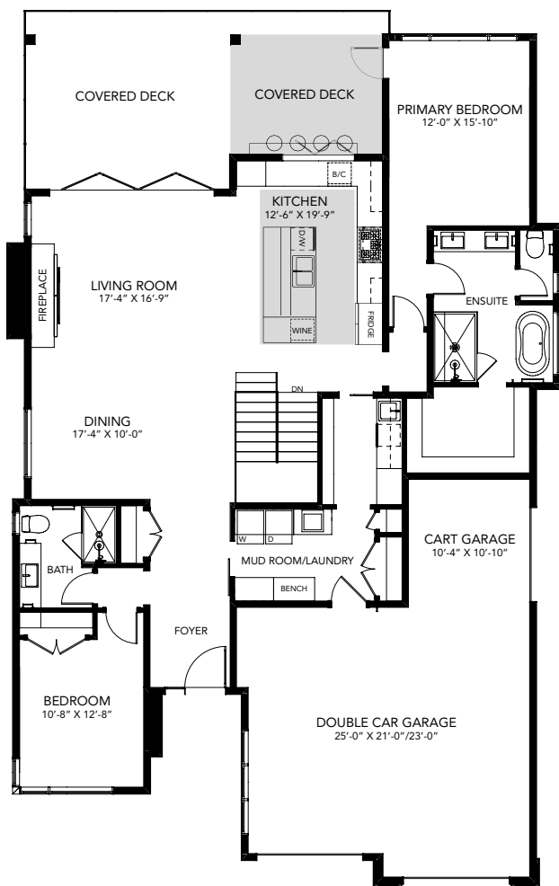
MAIN FLOOR AREA 1,913 SQFT
